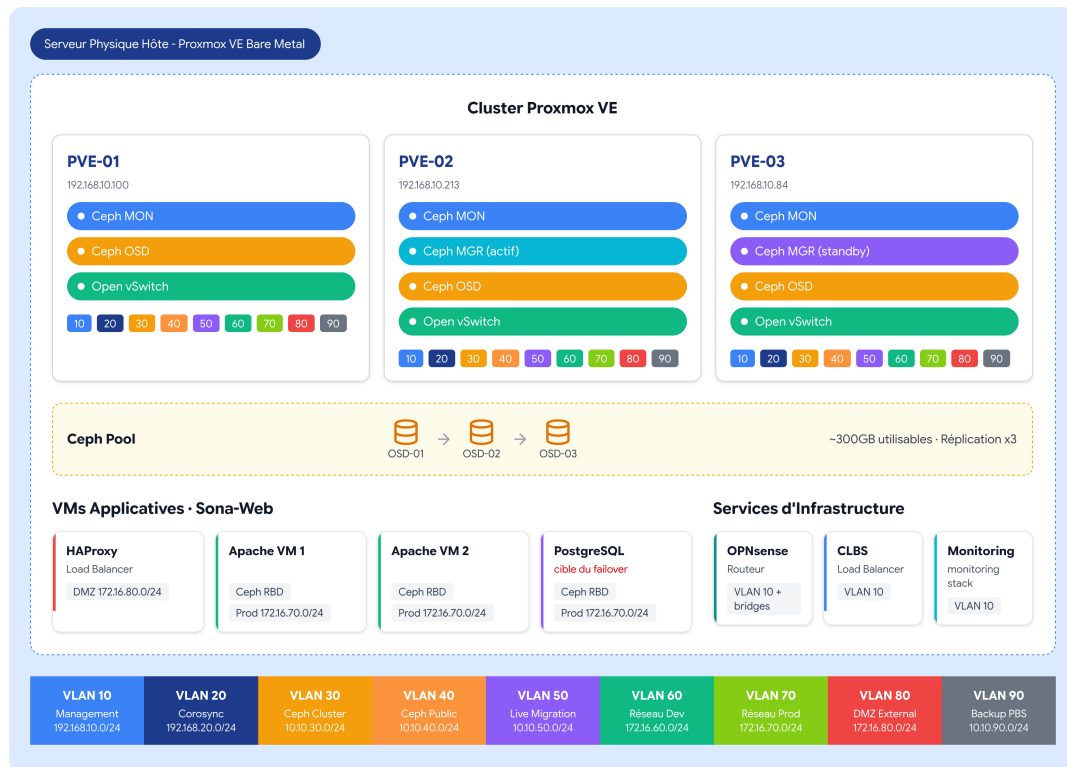
FIGURE III.1 – Architecture Globale de l'Infrastructure HCI
