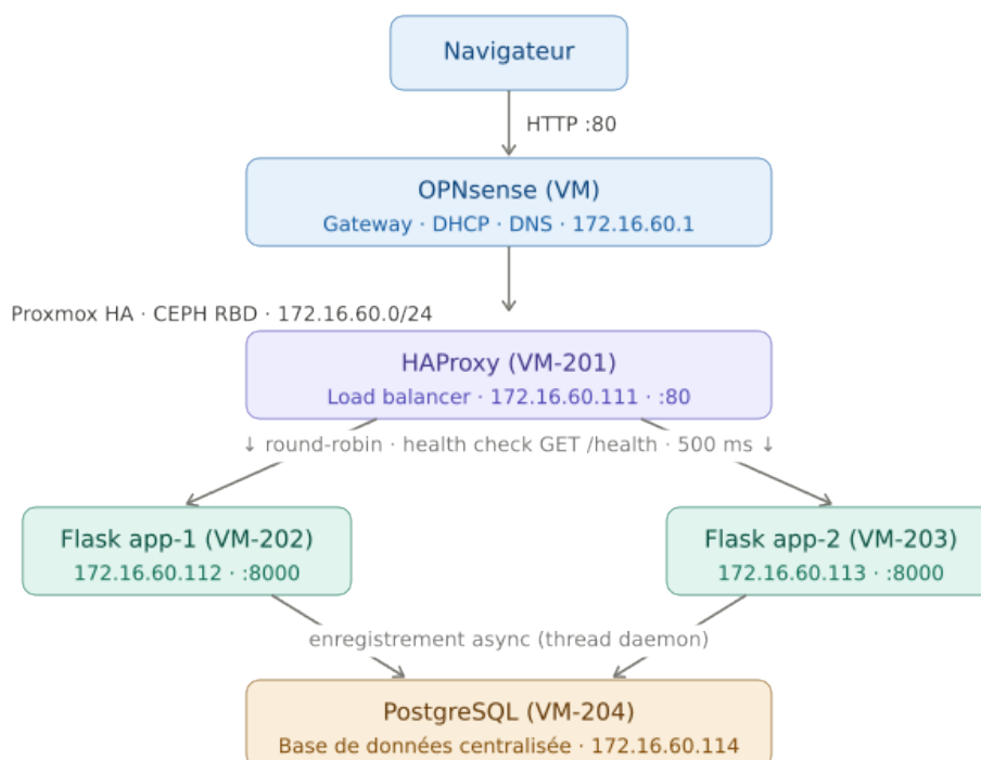
FIGURE III.3 – Architecture Applicative Sona-Web
