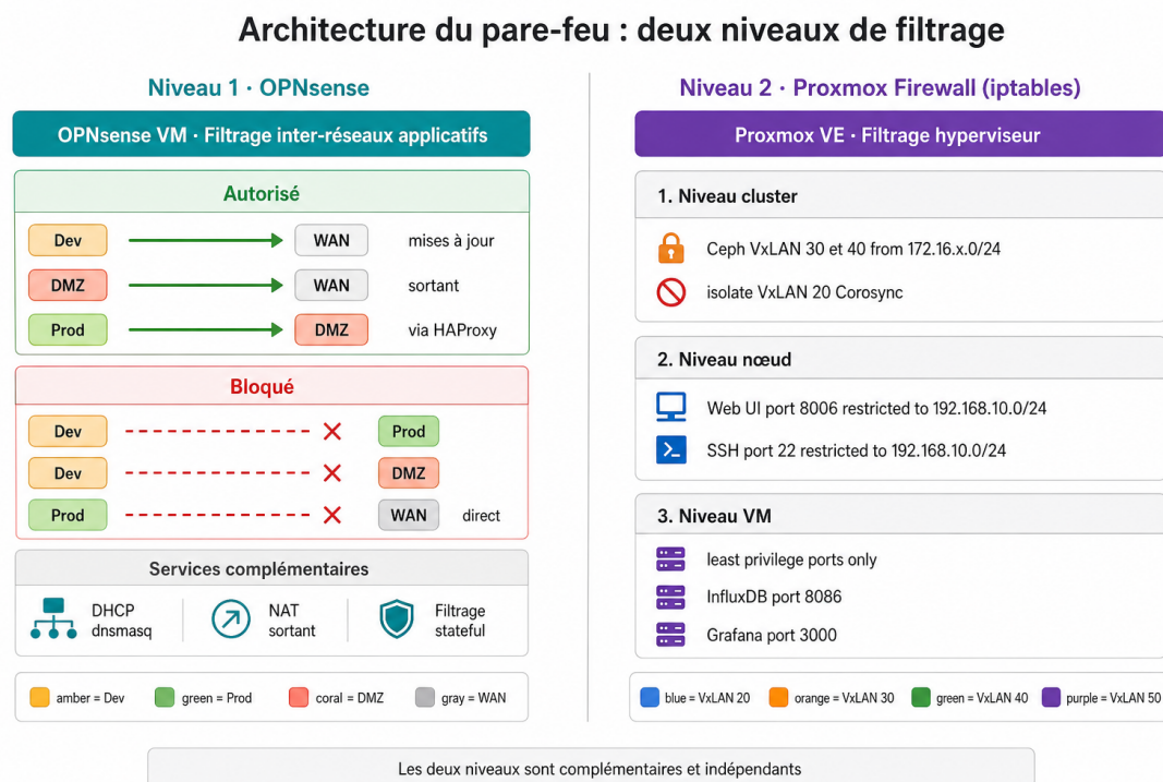
FIGURE III.5 – Architecture du Pare-feu : OPNsense et Proxmox Firewall
